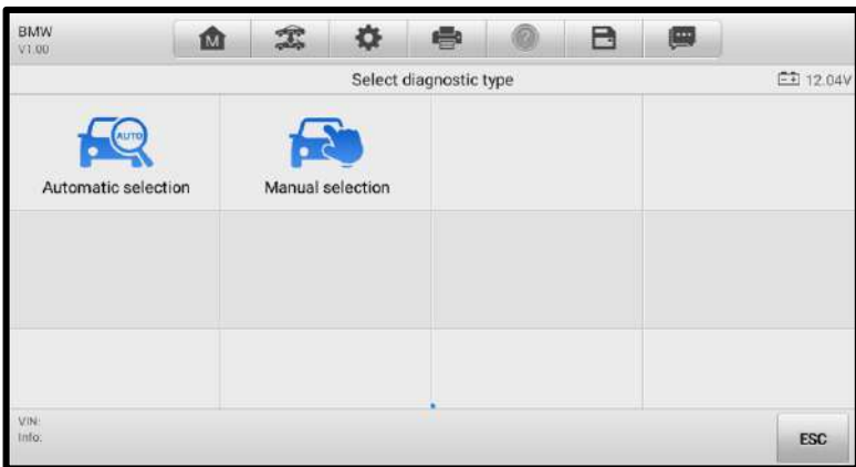
Figure 4-10 Selection Screen
