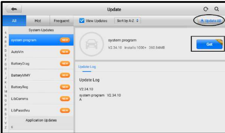
Figure 9-2 Update Screen 2
